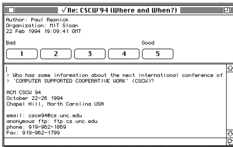
Fig. 2 (showing the user interface for GroupLens and the ability to rate articles 1-5). 46
