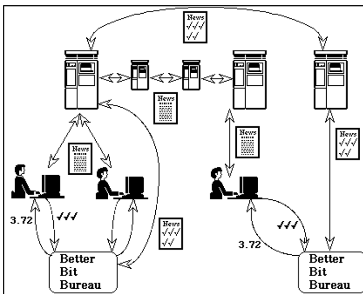
Fig. 3 (showing the architecture of the GroupLens system). 47
